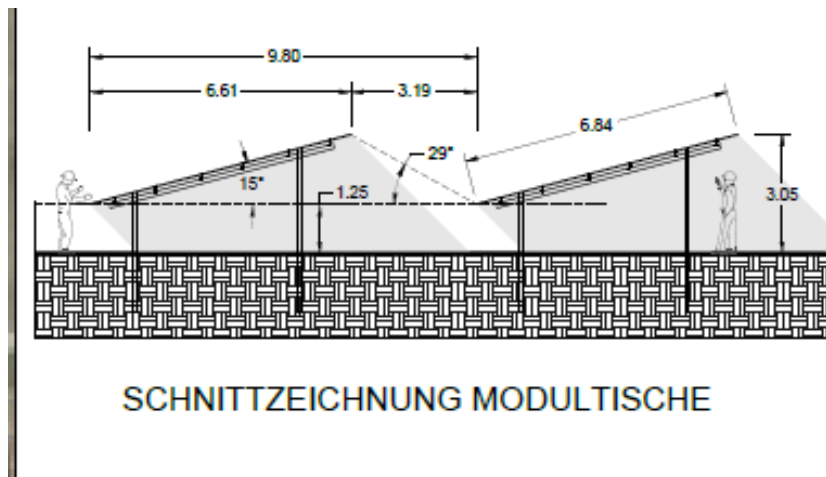
Abb.8: Skizze Modultisch (secureenergy)
